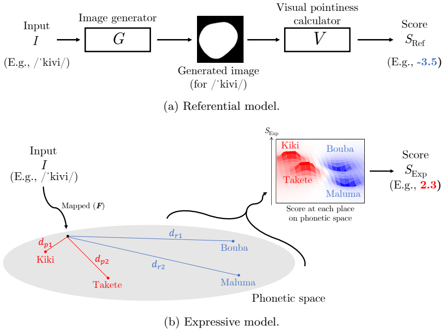
Fig. 4: Detailed procedure of calculating phonetic pointiness by the proposed models.
