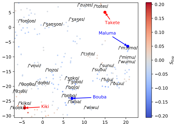
Fig. 9: Distribution of words in pronunciation sets as well as pseudo-words used in the phoneme experiment on our phonetic space, and corresponding phonetic pointiness scores for each pseudo-word calculated by the expressive model.
